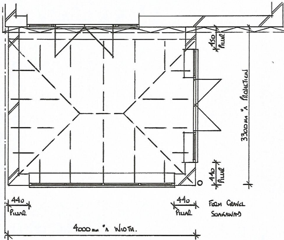
PROPOSED REAR PLAN VIEW
